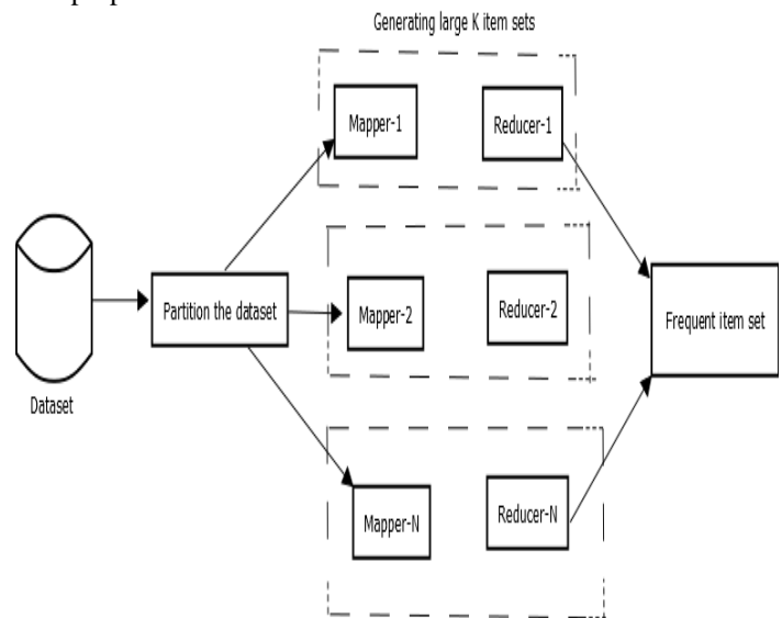
Figure 1 : System Architecture
