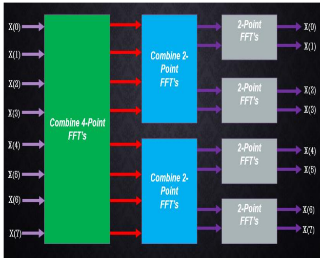
Figure 8 Radix-2 mechanism of FFT
