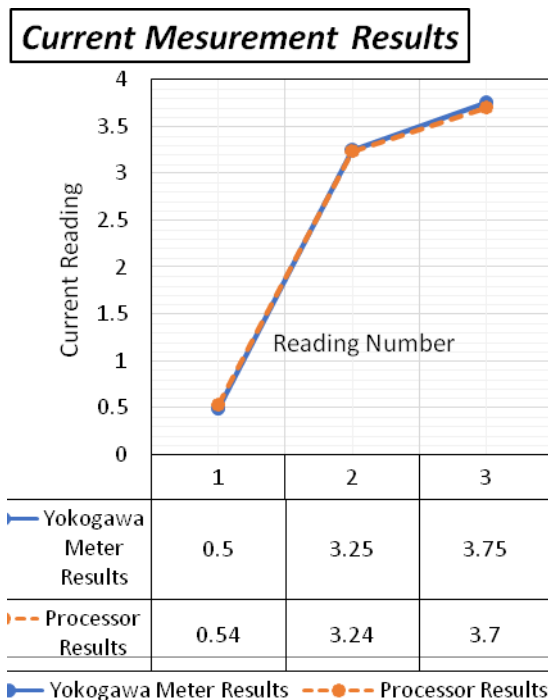
Figure 12 Current comparison between microcontroller and meter reading
