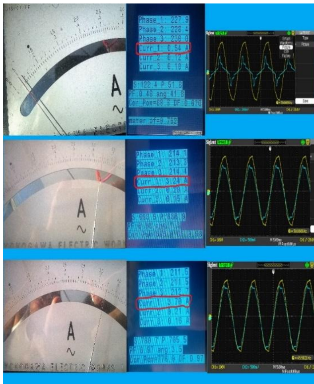
Figure 11 Current Measurement on microcontroller The graph of current reading is shown in figure 12.
