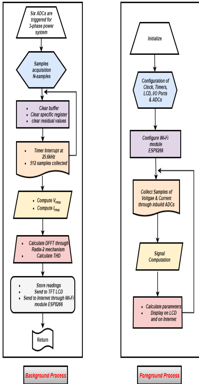
Figure 7 Flow chart of software implementation
