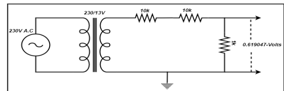
Figure 1 Schematic of voltage sensor's connection
