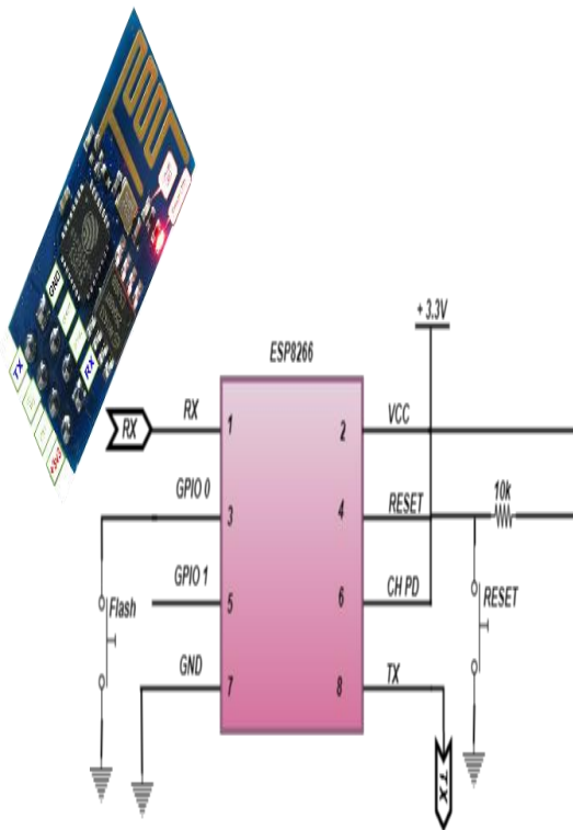
Figure 5 Schematic of ESP8266 Wi-Fi module
