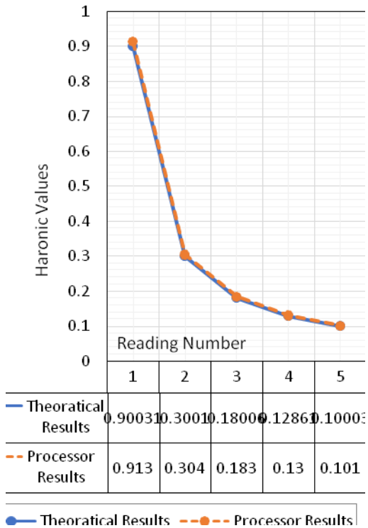
Figure 16 Comparison of harmonics calculation between microcontroller and theoretical results
