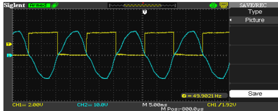
Figure 4 Output of zero crossing detector
