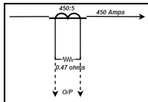
Figure 3 Schematic of current sensor's connection
