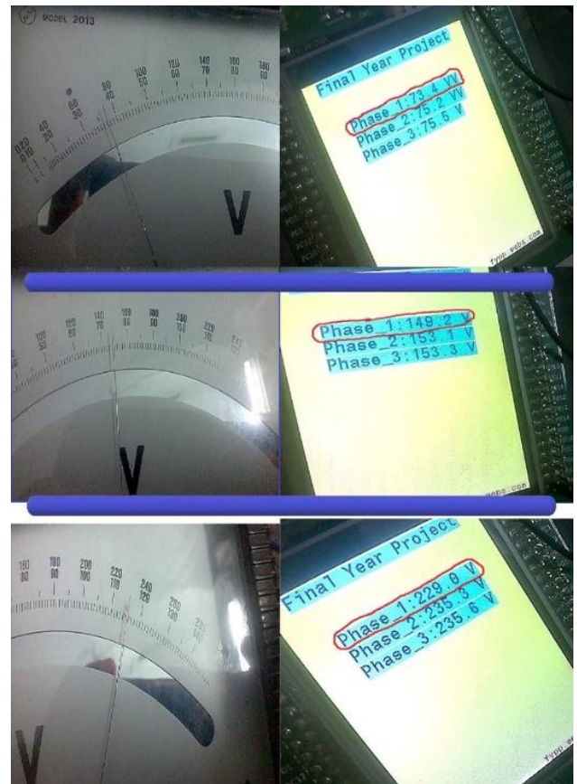
Figure 9 Voltage reading on microcontroller
