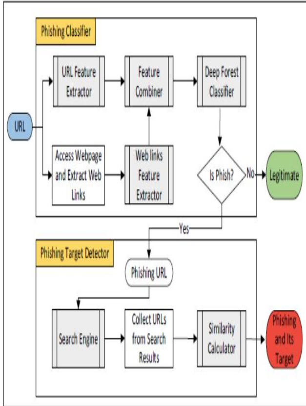
Figure 2. Overview of the proposed work
