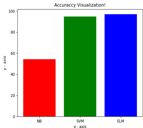
Figure 9: Accuracy Visualization
