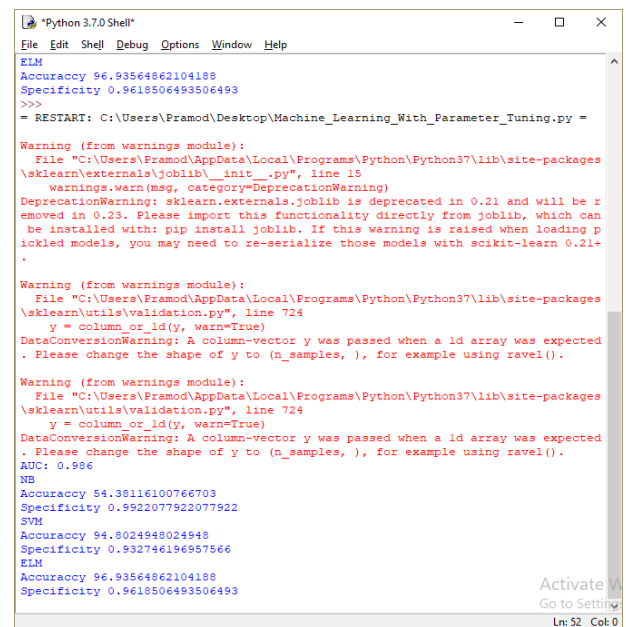
Figure 8: Accuracy Output
