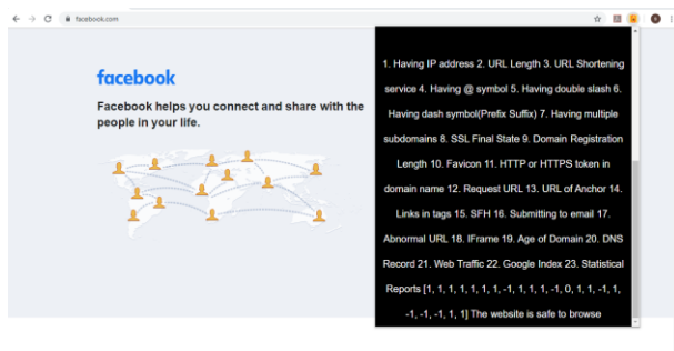
Figure 6: Normal Website Result
