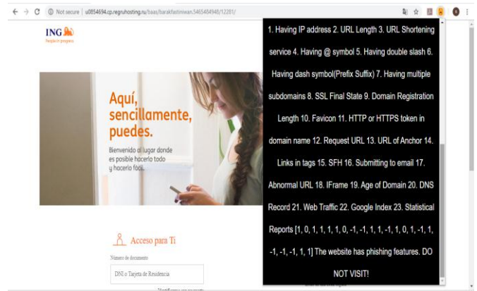
Figure 7: Phishy Website Detection
