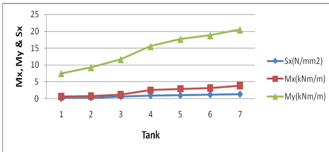
Graph 1 Moments & Shear forces behavior in soil pressure + wind pressure + surcharge.
