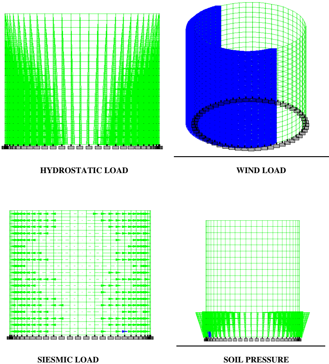
Figure 3.2 – Loads Behavior on Tanks
