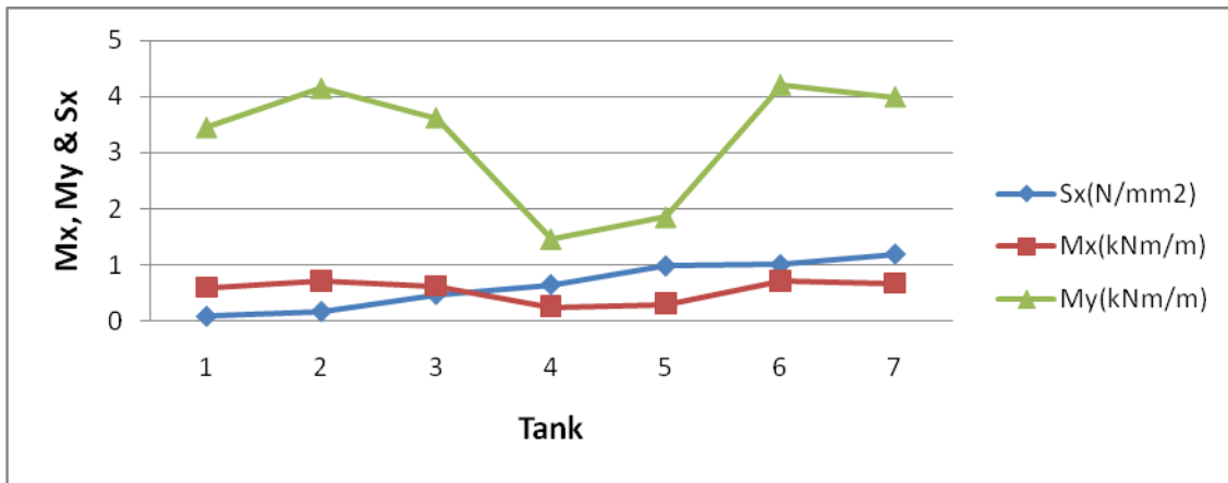
Graph 2 Moments & Shear forces behaviour in Wind Pressure + surcharge.
