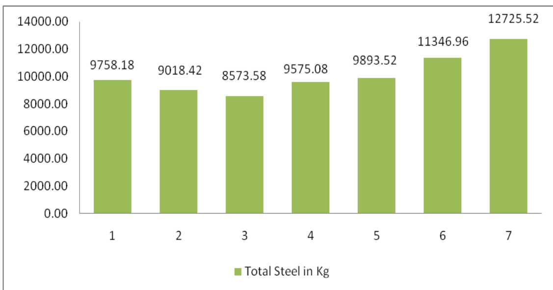
Graph 3 - Quantity of Steel in all Seven Tanks
