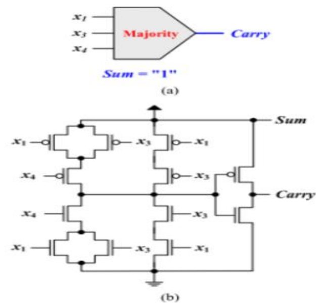
Fig. The proposed approximate 4:2 compressor (a) Block diagram. (b) Circuit design.
