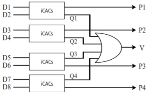
Fig. 3. Structure of an approximate tree compressor with eight inputs.
