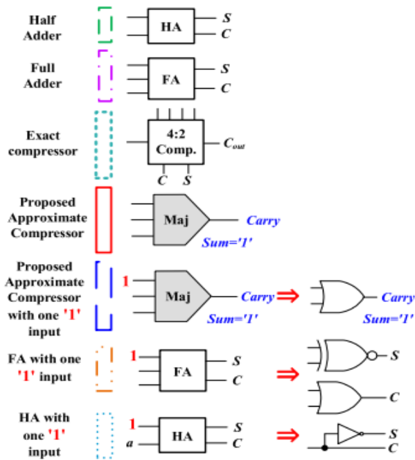
Fig. Partial product reduction circuitry of the proposed approximate multiplier.
