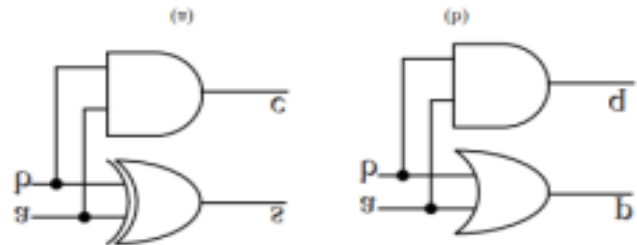
Fig. (a) Accurate half adder and (b) incomplete adder cell.
