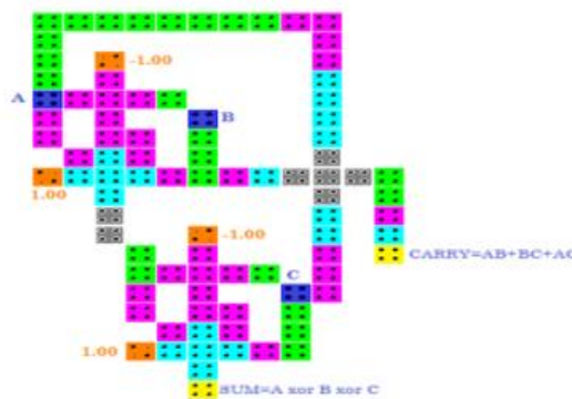
Figure QCA layout of Full Adder.
