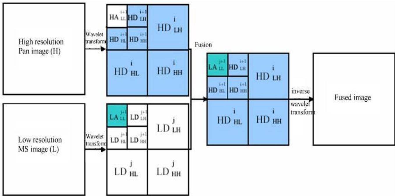
Figure 2. Generic flowchart of wavelet-based image fusion
