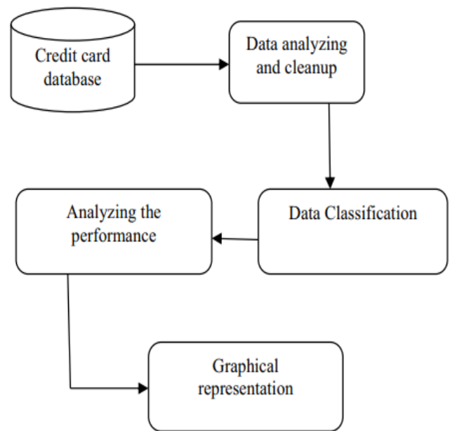
Fig 3: SYSTEM ARCHITECTURE
