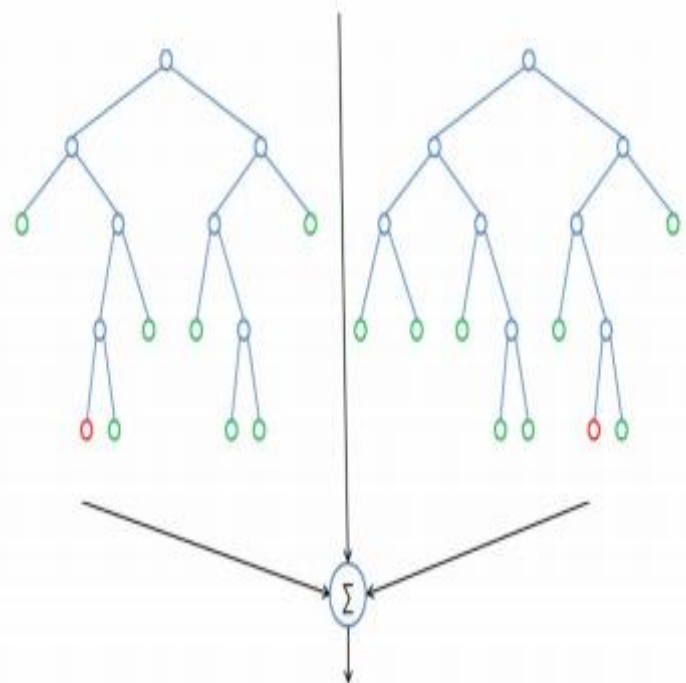
Fig 1: Decision tree
