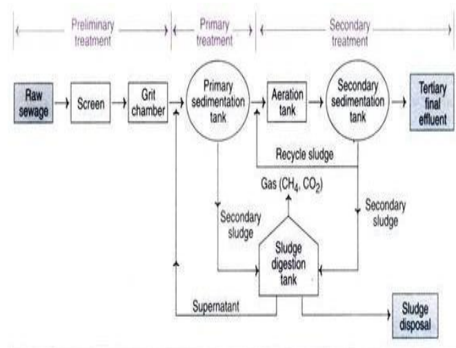
Fig.2 Shows The Conventional Flow Diagram Of Sewage Treatment Plant.
