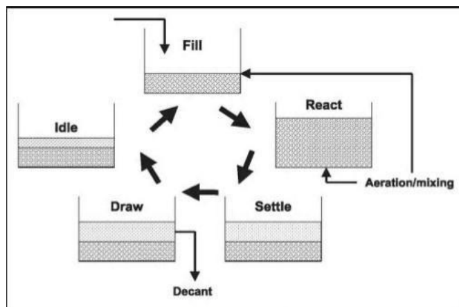
Fig.1 Show The Various Phases in SBR
